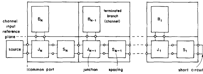
Fig. 6 The multiplexer configuration under consideration. J_1, J_2, \dots, J_N are arbitrarily defined 3-port junctions, B_1, B_2, \dots, B_N are terminated branches or channels which may each be represented in reduced cascade form, and S_1, S_2, \dots, S_N are usually waveguide spacing elements.
