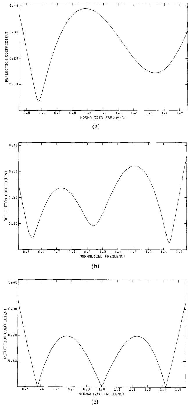
Fig. 5. (a) Response of the three-section transmission-line transformer at the starting point x_1^0 . The initial sample points are 0.5, 0.8, 1.2, and 1.5. The uniformly spaced (with the step length of 0.1) search points are 0.5, 0.6, ..., 1.5. The sample points selected by the algorithm using cubic interpolation are 0.5, 0.884, 1.2, and 1.5. The edges of the frequency interval are kept as the sample points. The initial sample point 0.8 has been replaced by the point 0.884 since a maximum has been detected between 0.8 and 0.9. The sample point 1.2 has not been changed since no maximum has been found between points 1.2 and 1.3. (b) Response of the three-section transmission-line transformer after the first iteration of optimization. The sample points selected by the cubic interpolation search (with the step length of 0.1) are 0.5, 0.729, 1.210, and 1.5. Now the initial sample point 1.2 has been replaced by 1.210 since a maximum has been detected between points 1.2 and 1.3. The sample point 0.884 has been replaced by a new sample point 0.729 resulting from the maximum between 0.7 and 0.8. (c) Response of the three-section transformer at the solution. The sample points selected by the cubic interpolation search (with the step length of 0.1) before the last iteration of optimization are 0.5, 0.770, 1.230, and 1.5.
